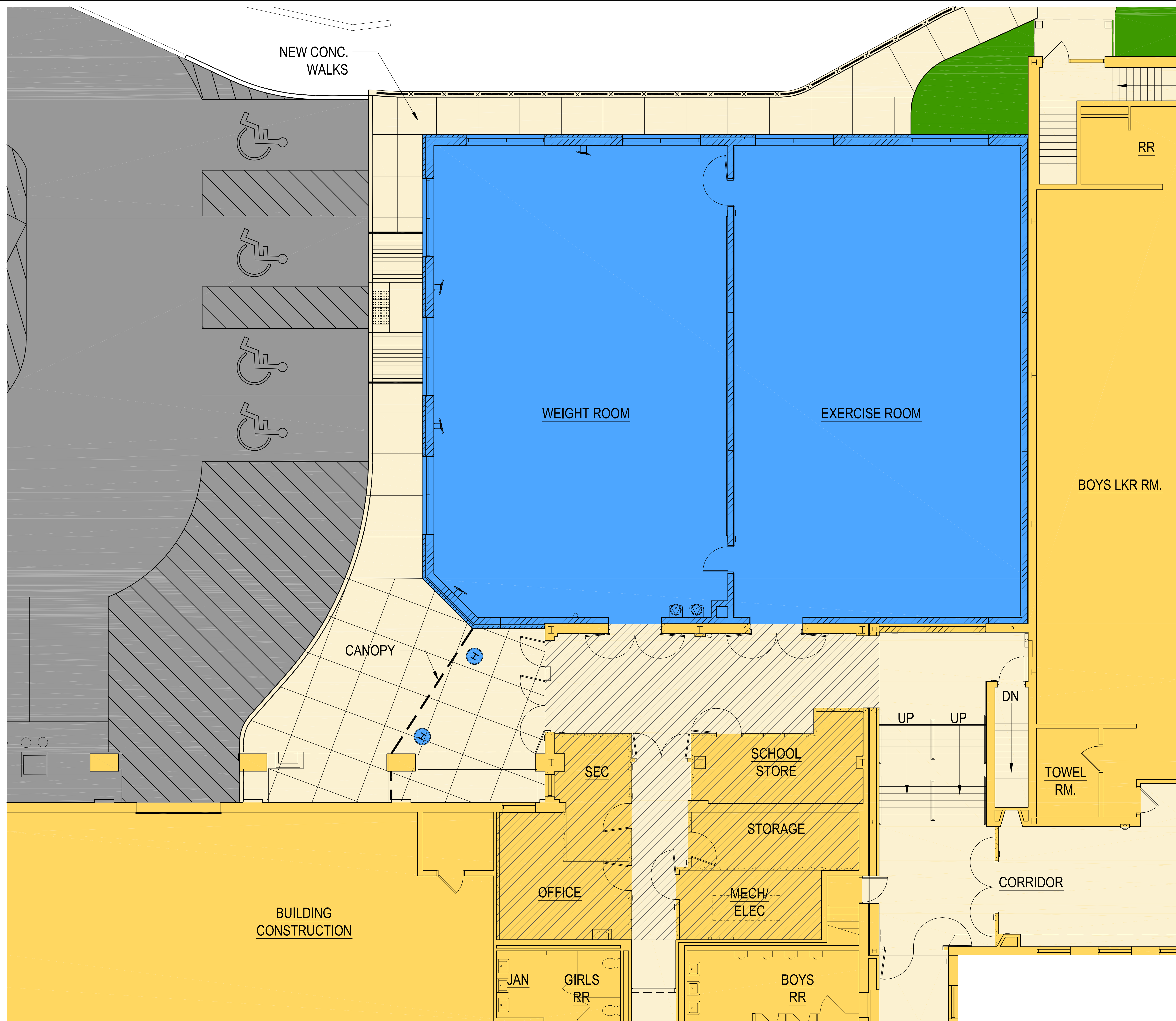
PARTIAL GROUND FLOOR PLAN NTS
